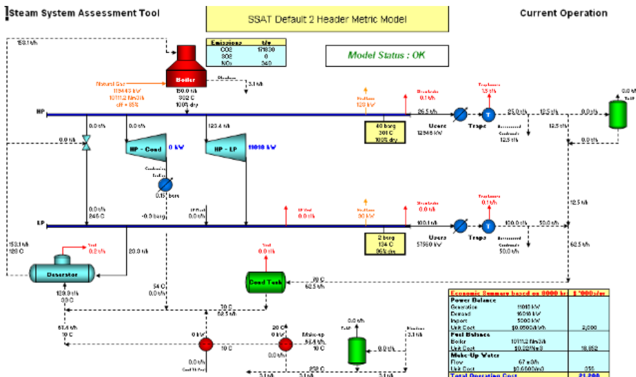
Figure 43: Example – Steam System Model
