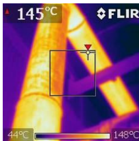
Figure 38: Thermal Images captured during a Steam System Assessment
