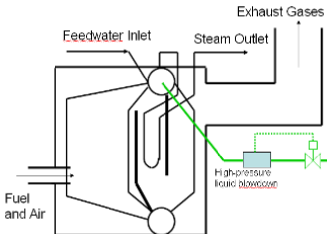
Figure 15: Automatic Boiler Blowdown Controller
