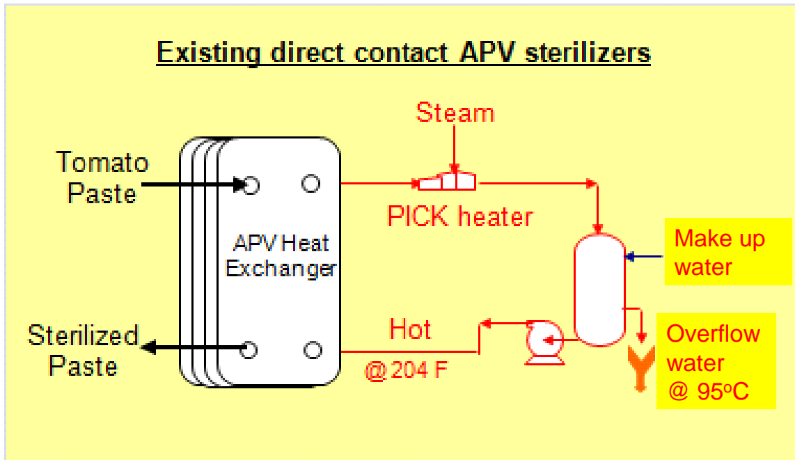
Figure 46: Process Flow Schematic of Original Evaporator Paste Sterilizer System
