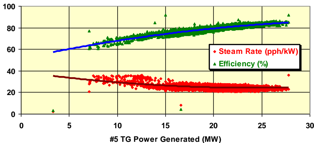
Figure 42: Example – Steam Turbine Operating Efficiency Curve
