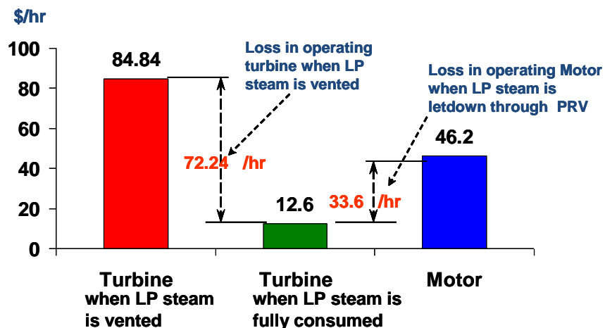
Figure 49: Operating Cost Impact & Optimization for ERC at the Refinery
