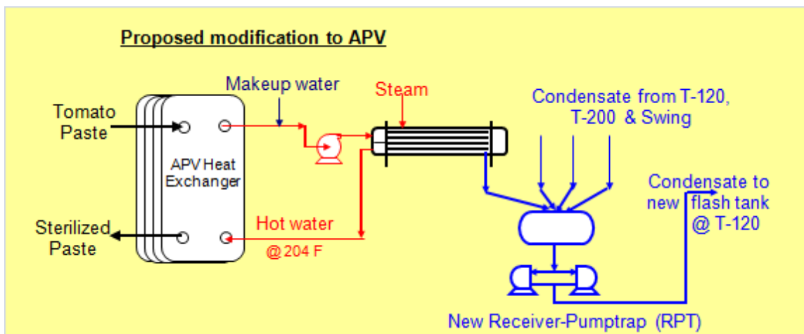
Figure 47: Process Flow Schematic of Improved Evaporator Paste Sterilizer System
